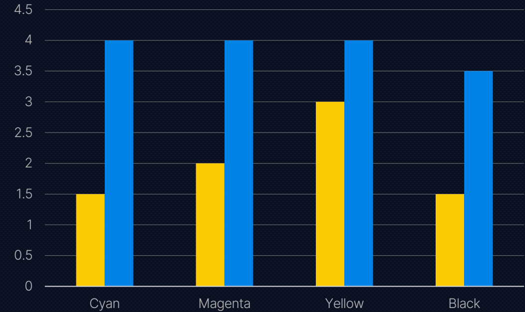
RUB FASTNESS ACCORDING TO ISO 105-X12 (WET)
